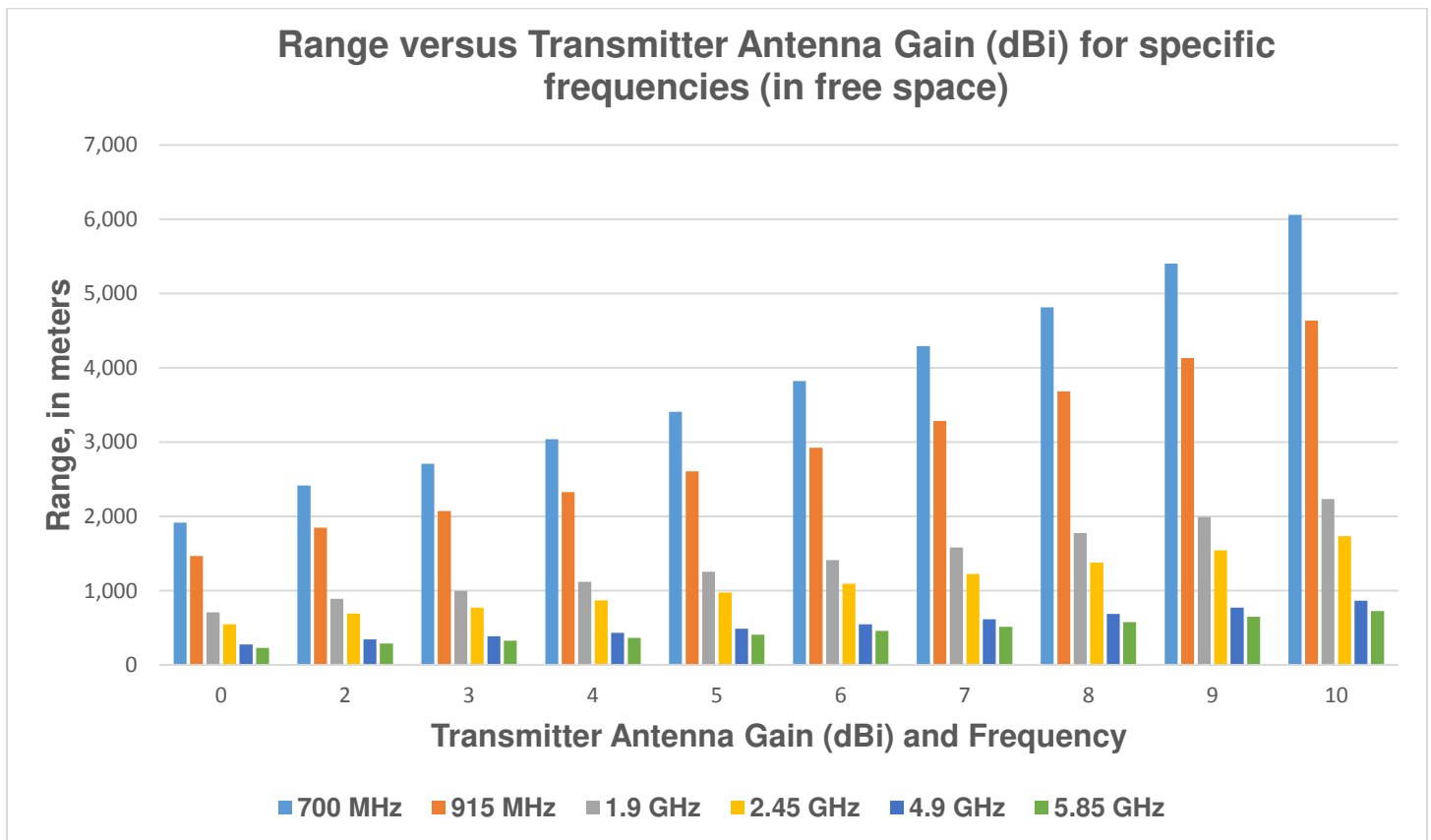
Fig. 2: Range based on antenna gain and frequency in free space
