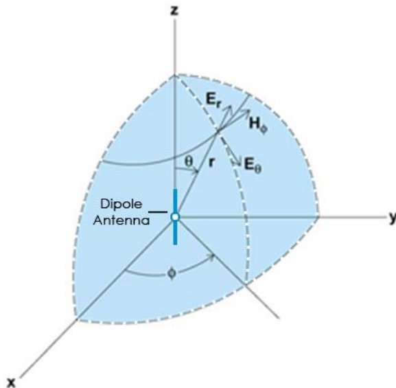
Fig. 3: Dipole antenna in spherical coordinate system
