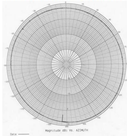
ECO8-2400 Series – Azimuth Plot
