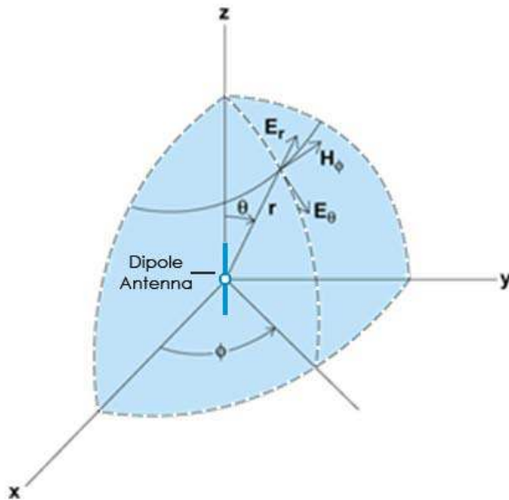
Fig. 3: Dipole antenna in spherical coordinate system
