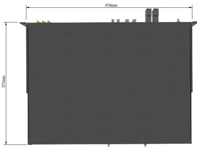
View - top
